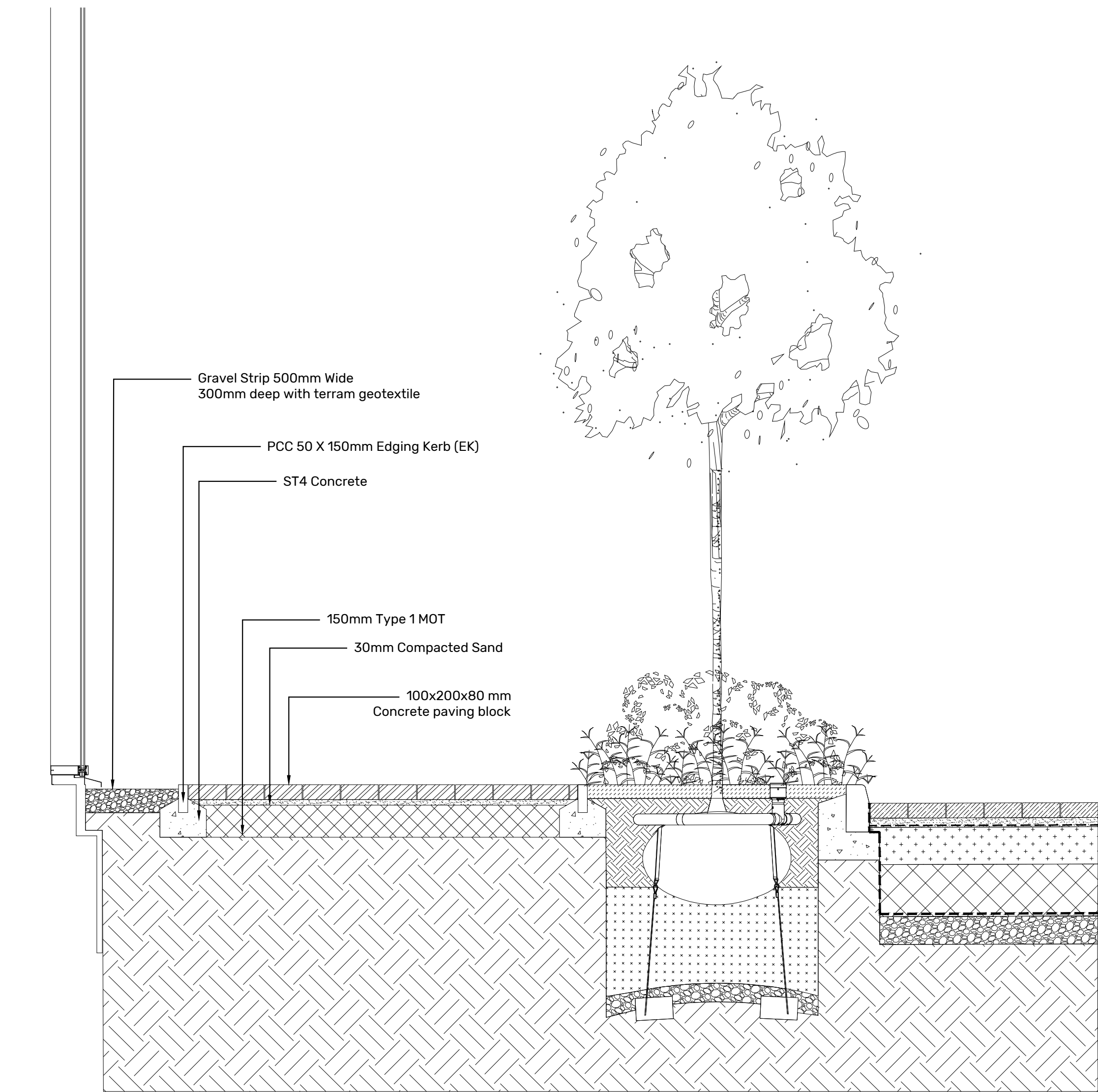
Typical Building Edge Section
